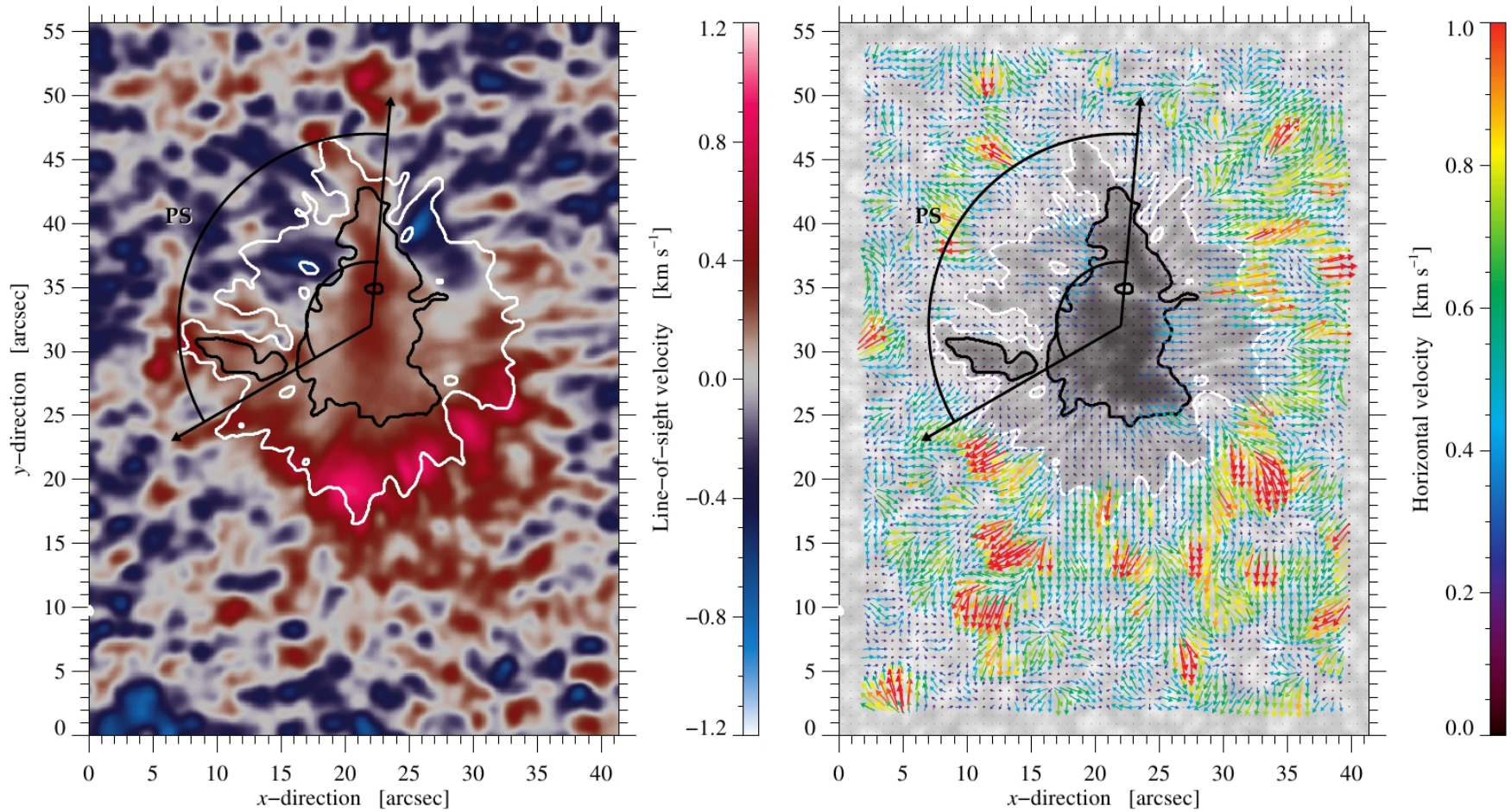
3D flow field from GREGOR GFPI - Doppler & LCT velocities
