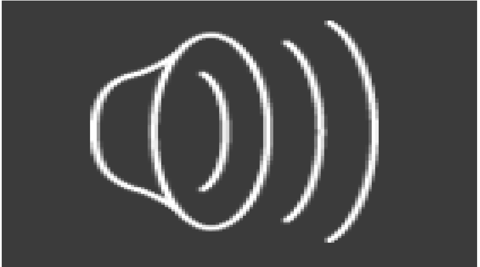
LOS velocity and line-core time-lapse movie
